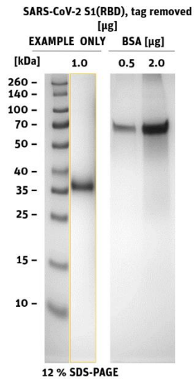
SDS-PAGE/Coll.Coomassie
