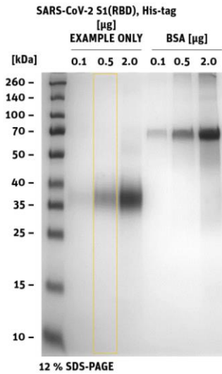
SDS-PAGE/Coll.Coomassie
